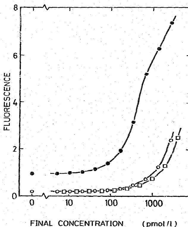
Fig.2. Fluorimetric detection of multi-FTC-PL using anti-fluorescein serum and FTC-G (closed circles) compared with that of multi-FTC-PL alone (open circles) and FTC-G alone (open squares). Total fluorescence signals are shown; the buffer background signal was 0.17 units.
